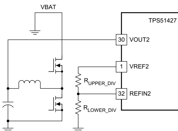
Figure 47. Channel2 Adjustable Voltage Configuration
